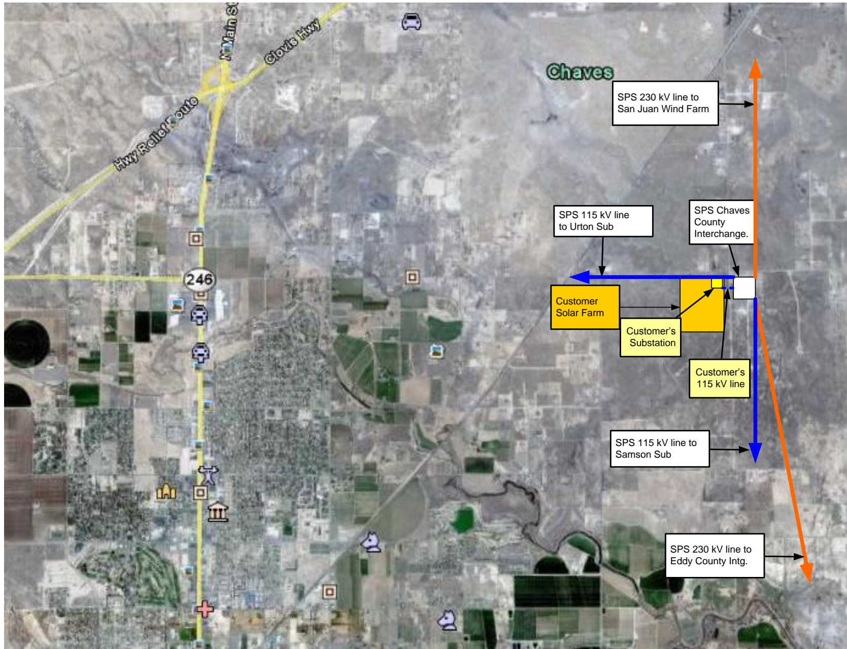
Figure A-1. Approximate location of proposed Solar Farm Facility and Interconnection Customer's 115 kV Transmission Line.
