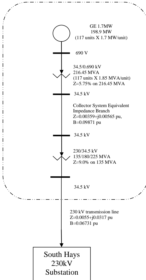
Figure 2: GEN-2009-008 Facility One-line Diagram
